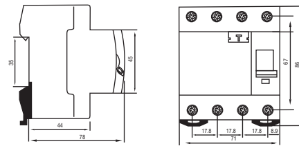
Overall & Installation Dimensions
